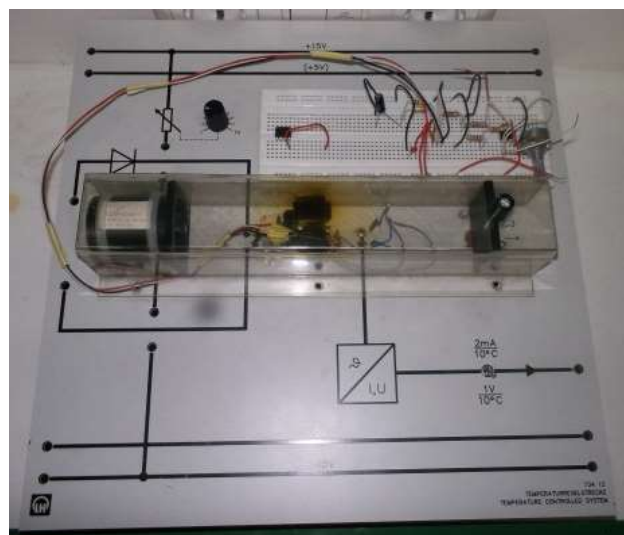
Gambar 4. Modul Temperatur Controlled System – Leybold 734 12
