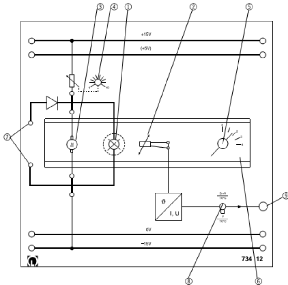
Gambar 3. Rangkaian plant
