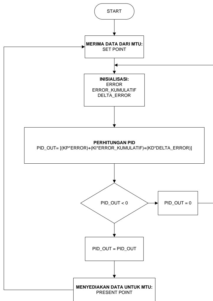
Gambar 5. Diagram alir program di RTU
