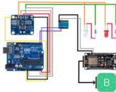
Gambar 2 Perancangan Hardware
