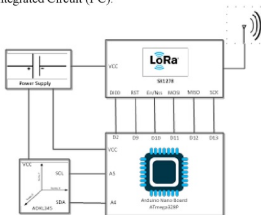
Gambar 2. Arsitektur Dasar Hardware Wearable Device Pengirim Data
