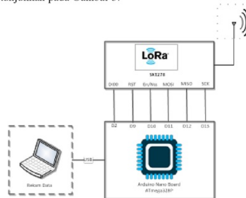
Gambar 3. Arsitektur Dasar Hardware Penerima Data Wearable Device
