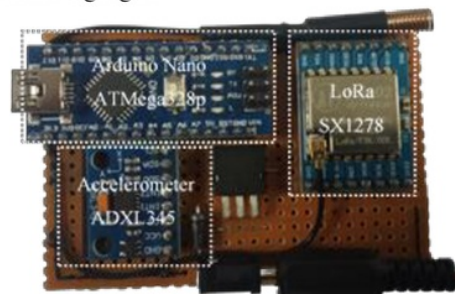
Gambar 4. Purwarupa Wearable Device Pengirim Data
